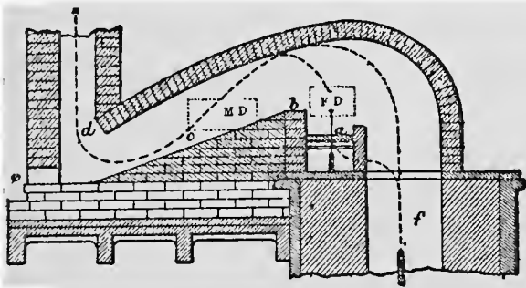
FIG. 13. THE REVERBERATORY FURNACE
